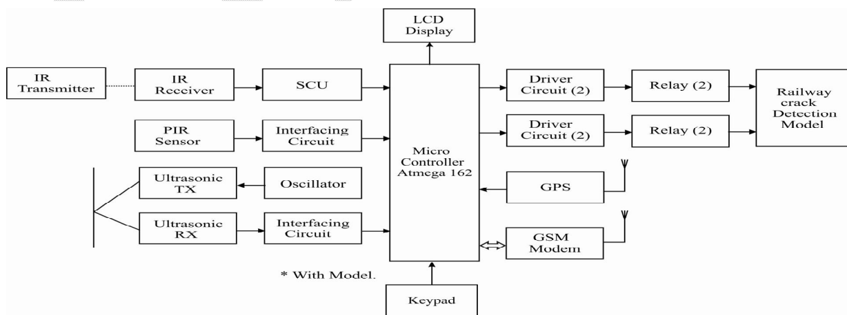
Fig 6: Block Diagram
