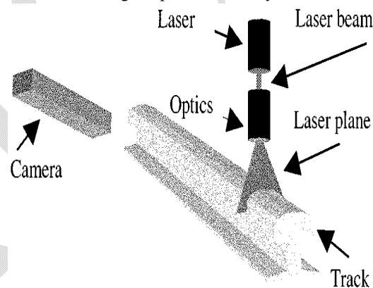
Fig 1: Detection System
